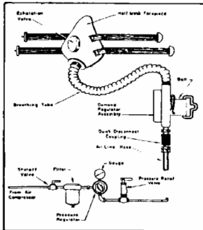
AIR LINE RESPIRATOR
