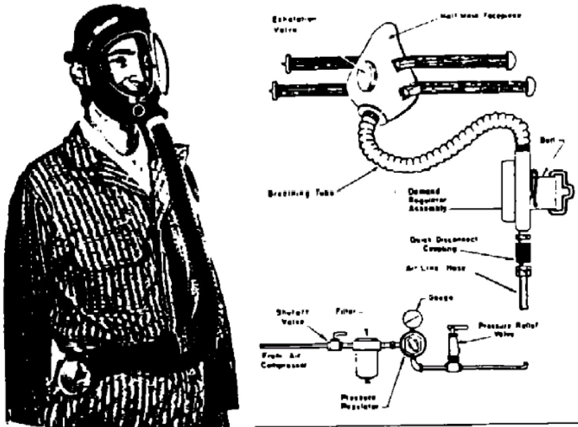
AIR LINE RESPIRATOR DIAGRAM SHOWS PARTS WITH FULL - FACE MASK Fig. 13
